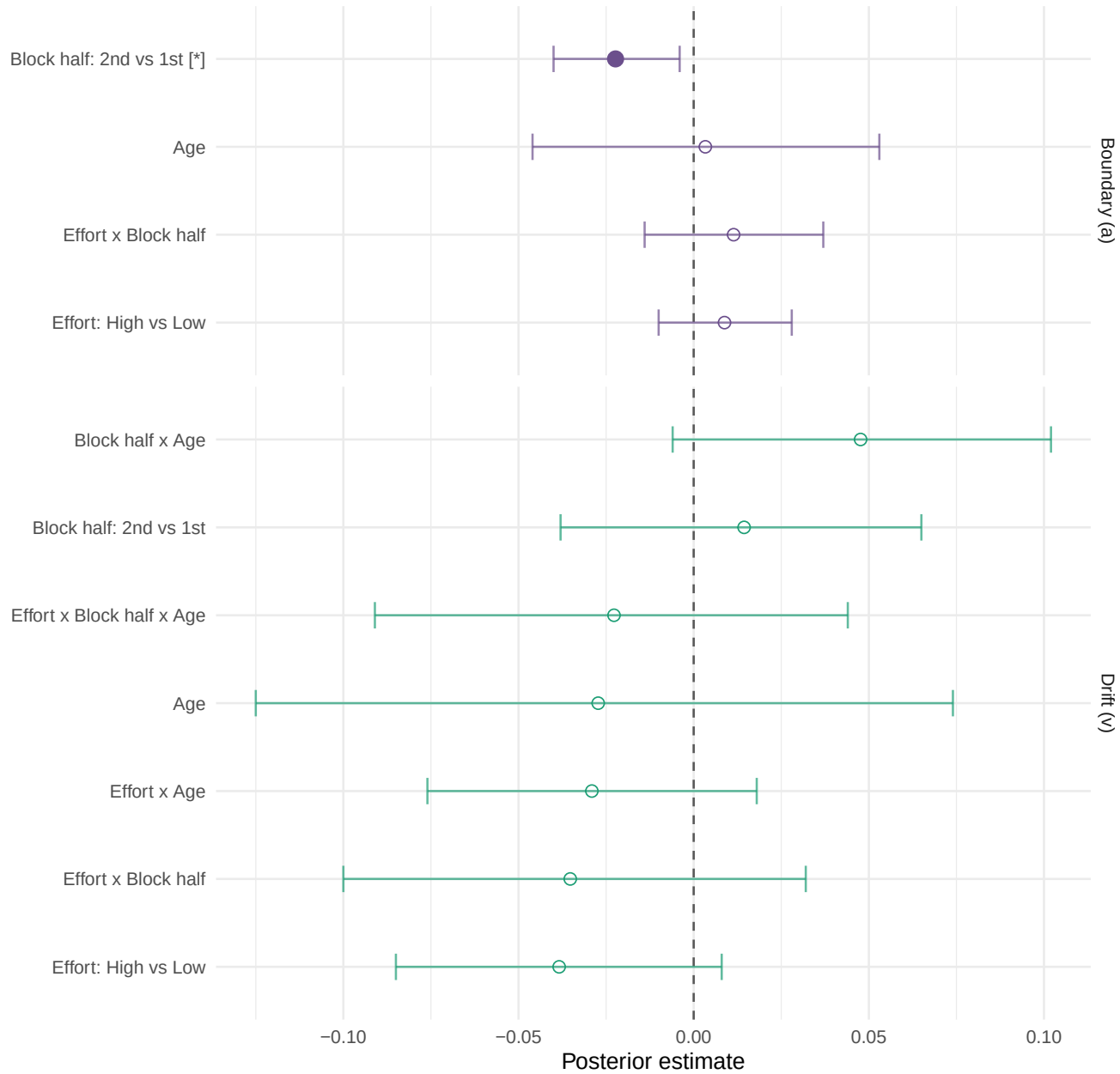
Coefficient estimates
