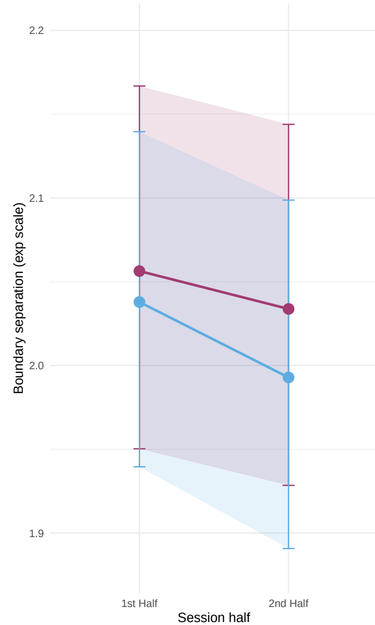
Boundary trajectories
